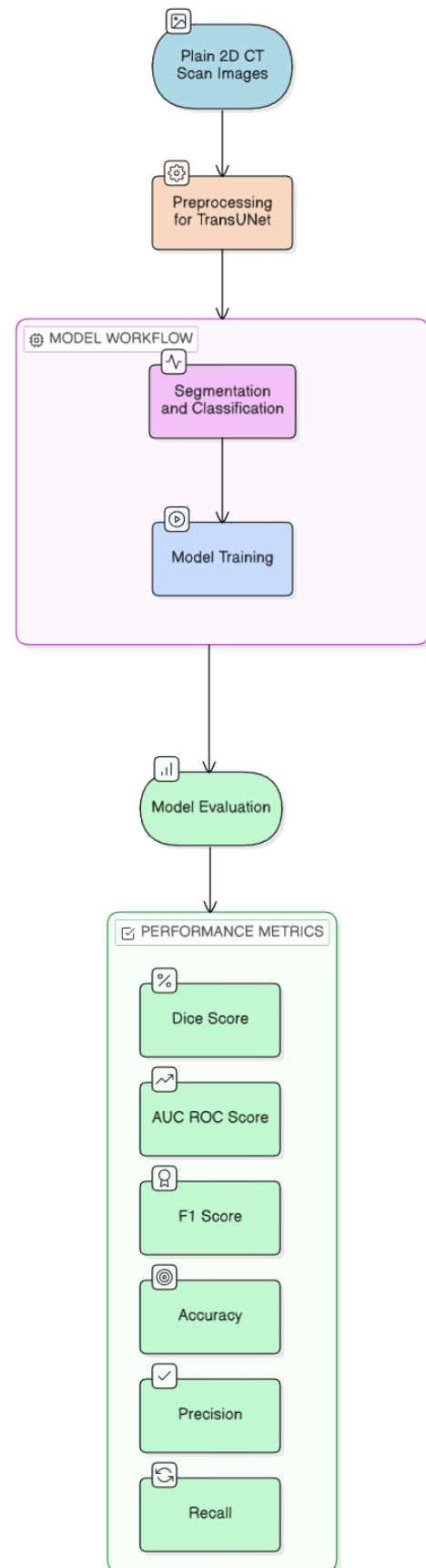
Fig 1. Proposed Methodology
